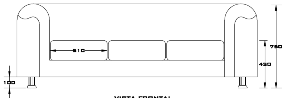
VISTA FRONTAL
