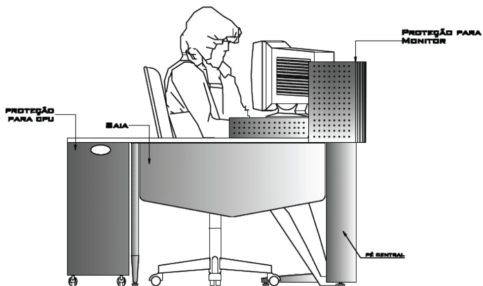
VISTA FRONTAL
